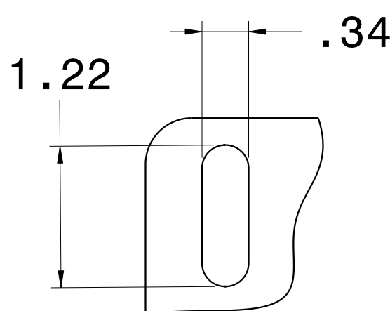
SLOT DETAIL 4X
