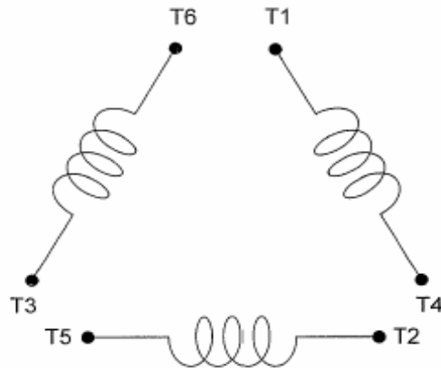
SCHEMATIC - Δ / Y CONNECTION
