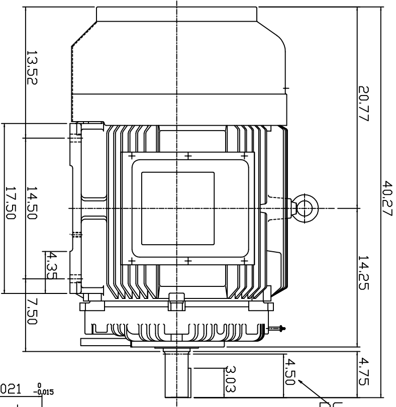
TOTALLY ENCLOSED FAN-COOLED TYPE, SQUIRREL-CAGE ROTOR
