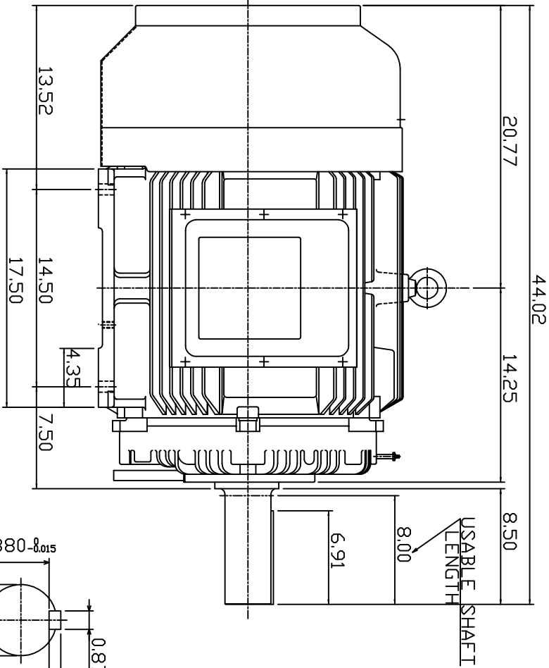
TOTALLY ENCLOSED FAN-COOLED TYPE, SQUIRREL-CAGE ROTOR
