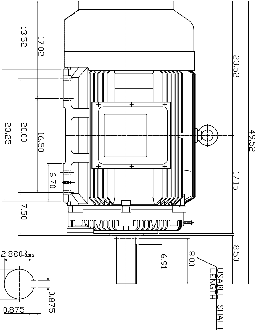
TOTALLY ENCLOSED FAN-COOLED TYPE, SQUIRREL-CAGE ROTOR
