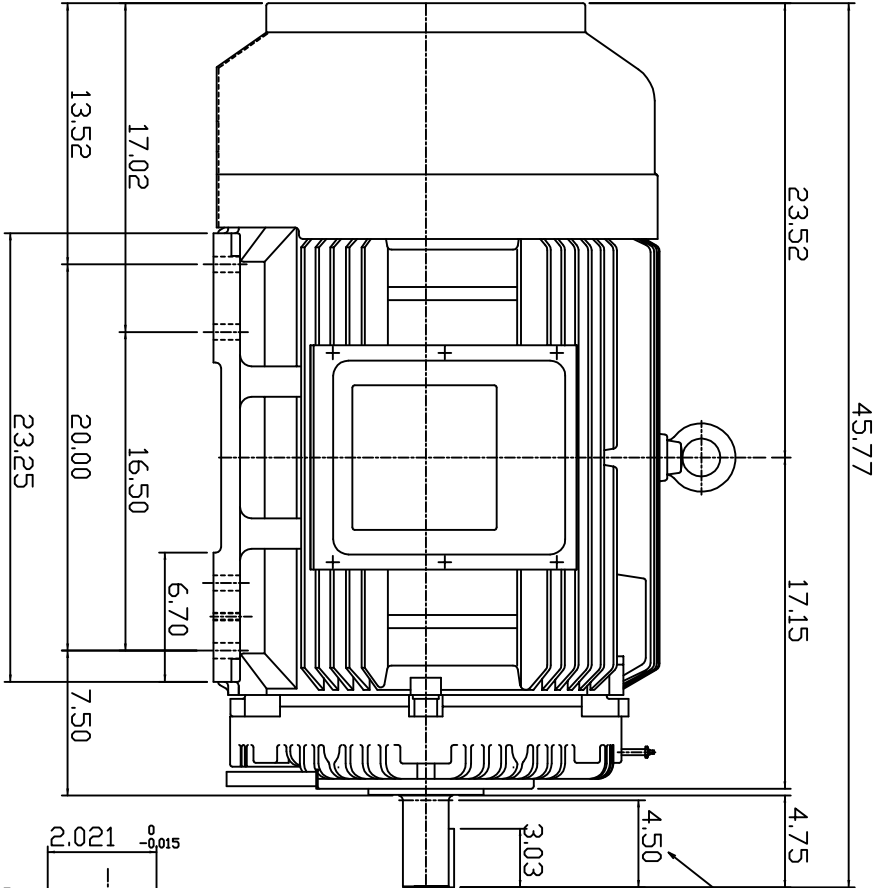
TOTALLY ENCLOSED FAN-COOLED TYPE, SQUIRREL-CAGE ROTOR
