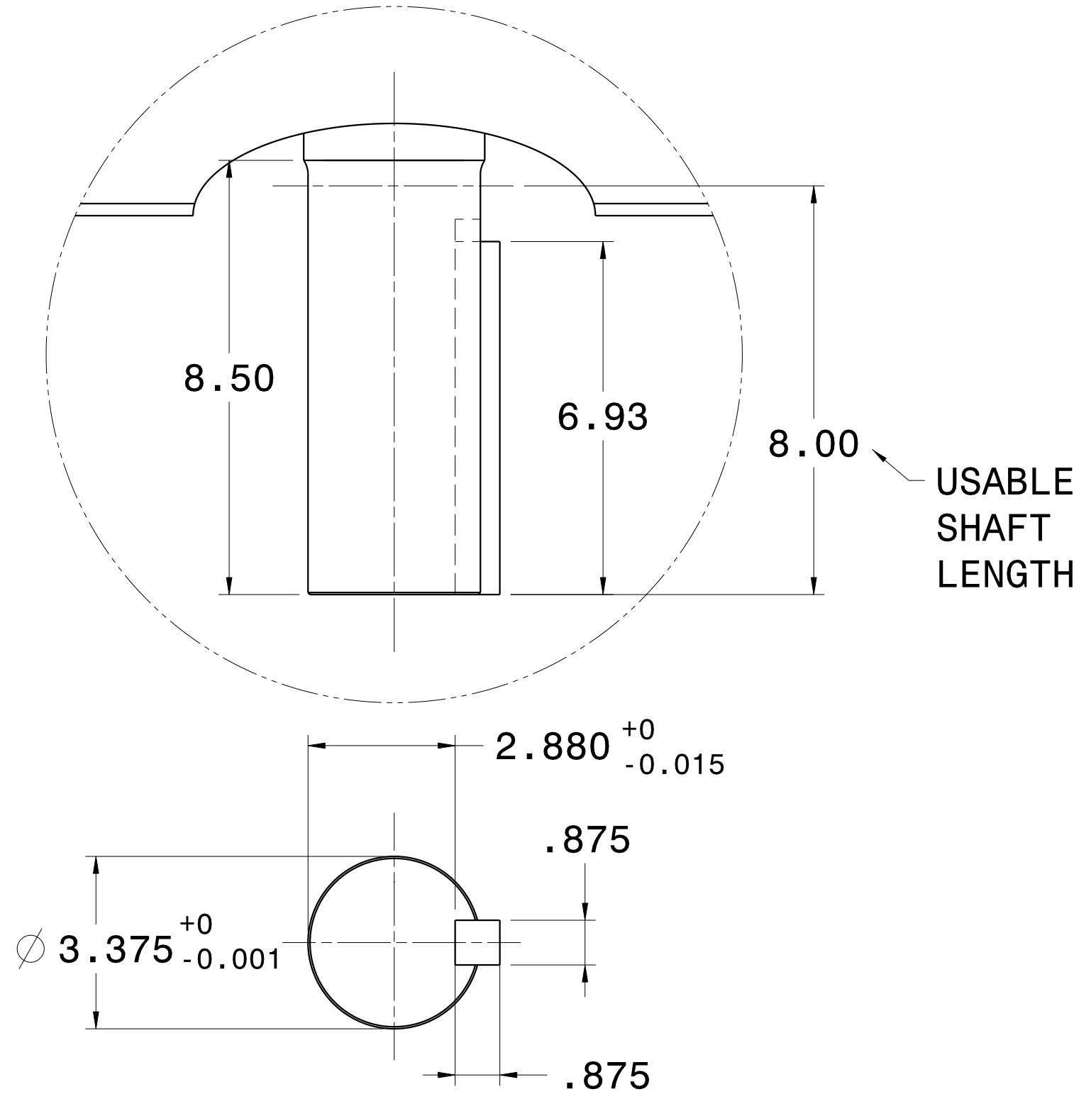
SHAFT DETAIL
