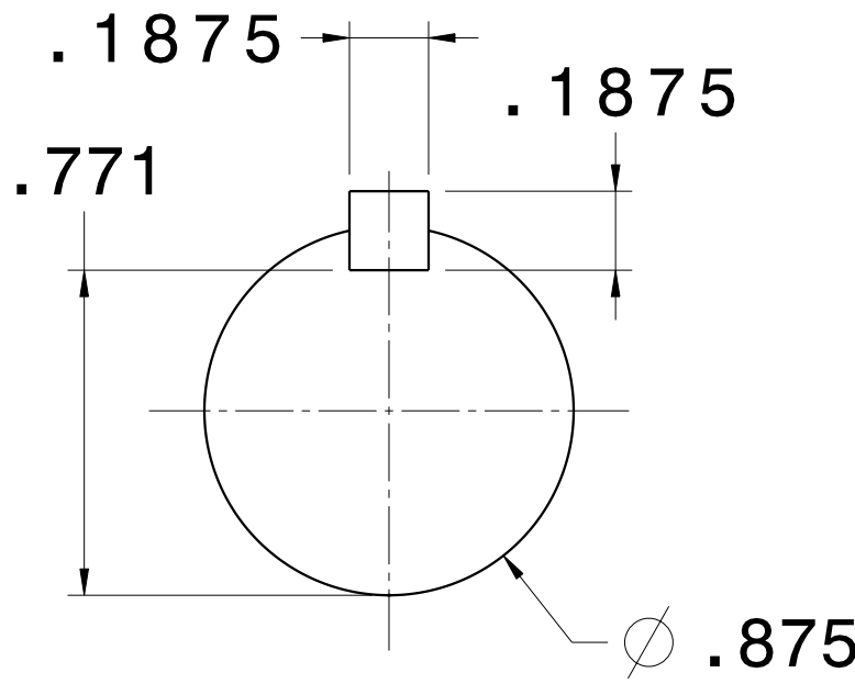
SHAFT END (ENLARGED VIEW)
