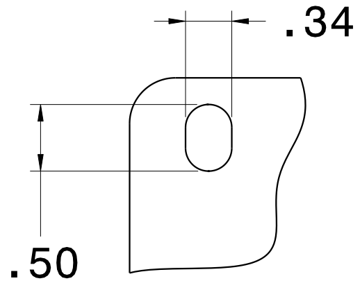
SLOT DETAIL 6X
