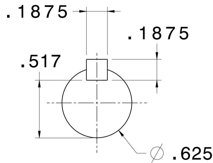
SHAFT END (ENLARGED VIEW)
