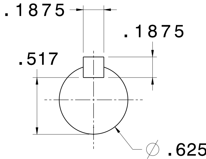
SHAFT END (ENLARGED VIEW)
