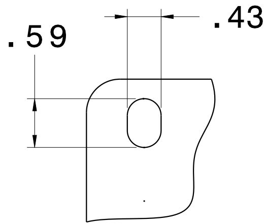
SLOT DETAIL
