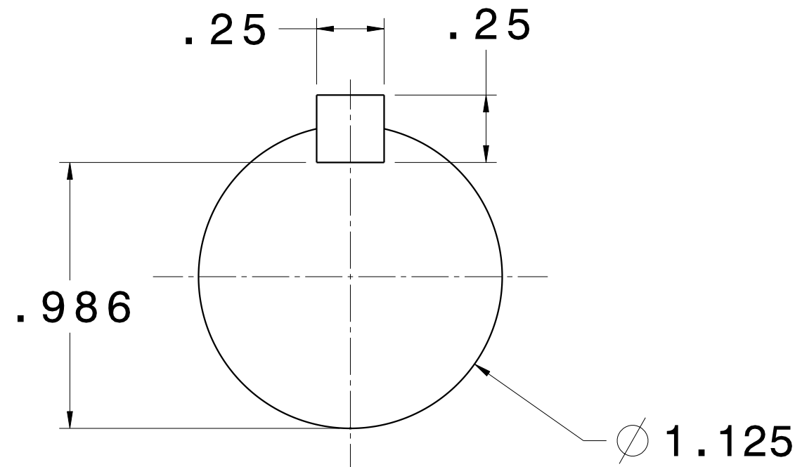
SHAFT END
