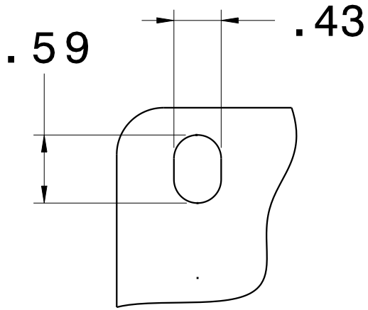
SLOT DETAIL
