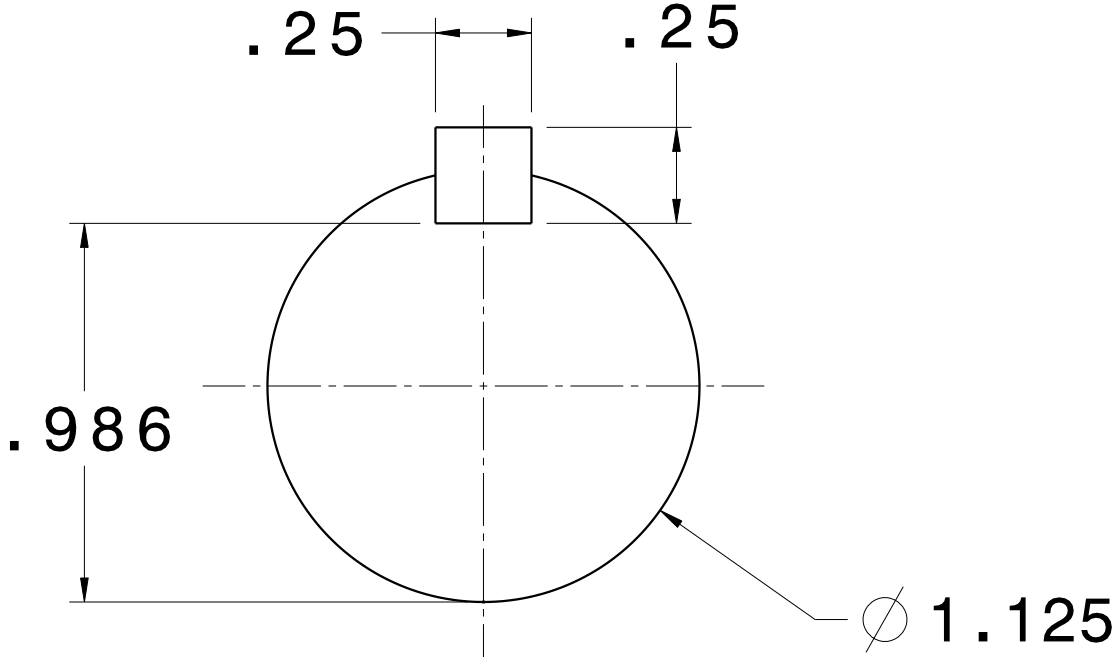
SHAFT END
