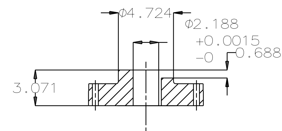
COUPLING [ENLARGED VIEW]
