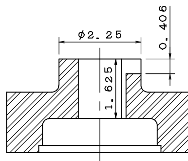
Coupling Dimension
