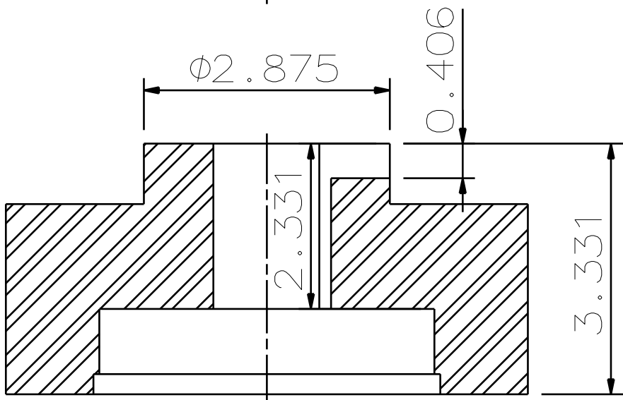
Coupling Dimension
