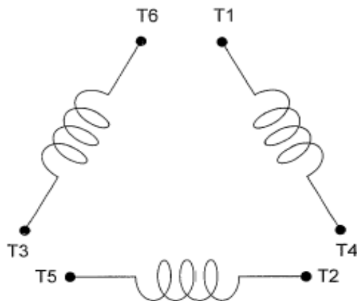
SCHEMATIC - \Delta CONNECTION
