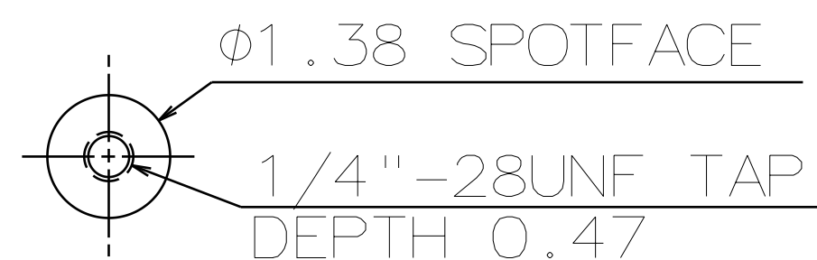
DETAIL A (PROVISION FOR VIBRATION SENSOR)
