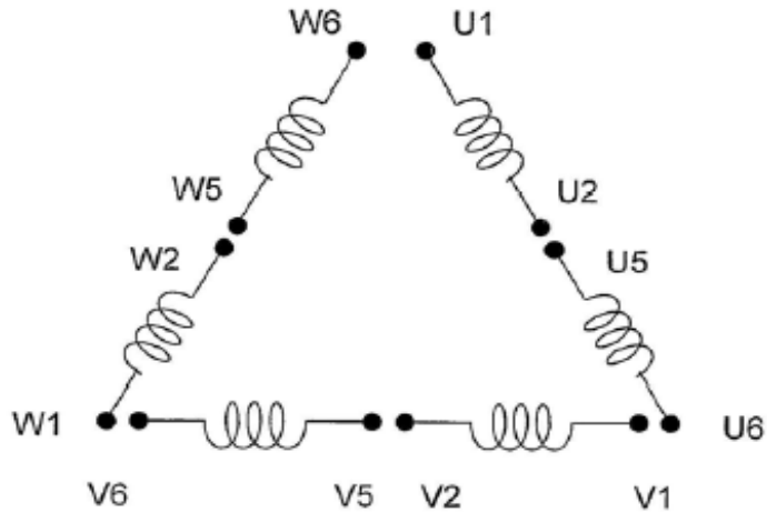
SCHEMATIC - \Delta / Y CONNECTION
