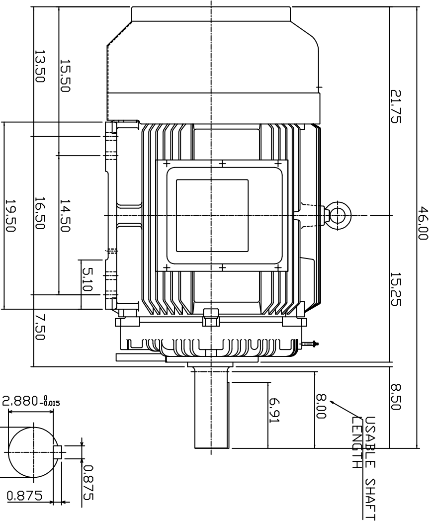
TOTALLY ENCLOSED FAN-COOLED TYPE, SQUIRREL-CAGE ROTOR
