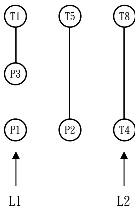
230V CW ROTATION
