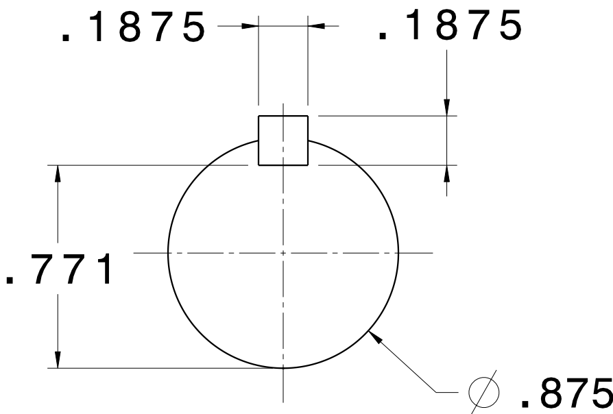
SHAFT END
