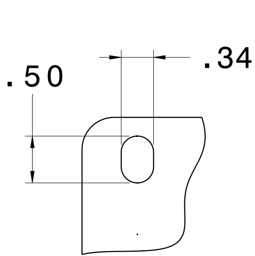
SLOT DETAIL
